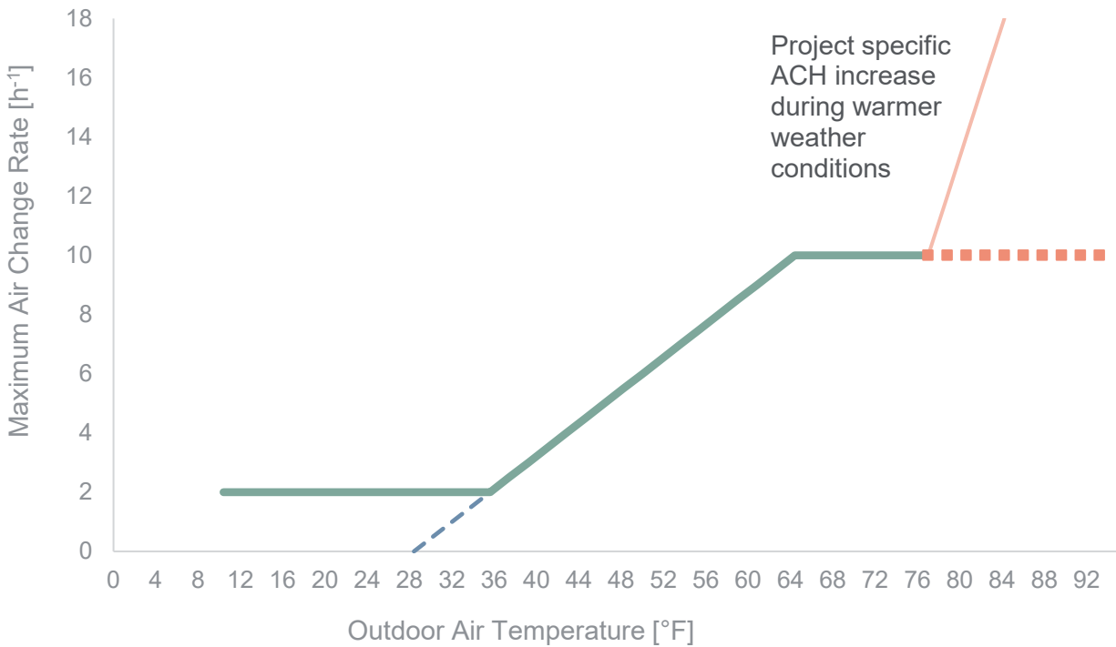
Figure 2 – The maximum allowable Air Change per Hour based on the Outdoor Air Temperature. Limiting the maximum ACH will provide a greater thermal comfort for the occupants.
